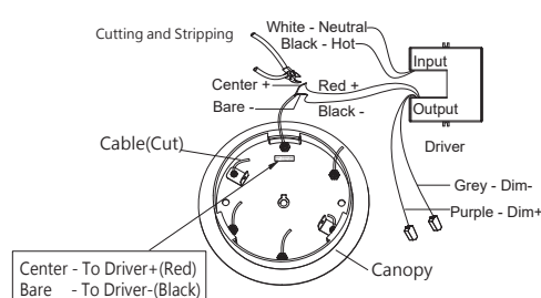
Fig.3 Driver Wires
